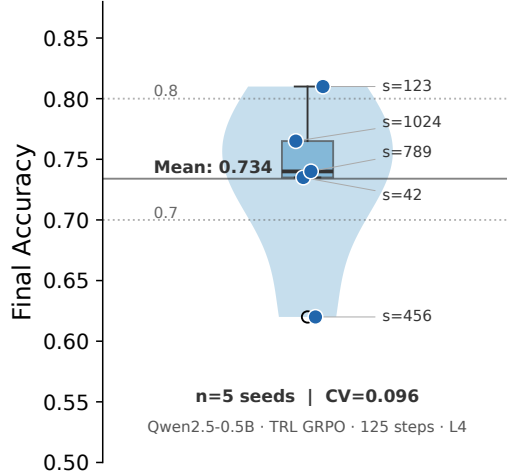
Figure 19: Cross-seed reproducibility for TRL GRPO on Qwen2.5-0.5B (GSM8K, 125 steps, NVIDIA L4). Five seeds show mean verifier score 73.4% with CV = 0.096. Violin plot shows the distribution; individual seeds are labeled. We report the five-seed spread rather than a null-hypothesis test: a t -test against 50% is not an appropriate null for GSM8K (a random-guess baseline is closer to 0% than 50%), so the low CV is the defensible finding here.
